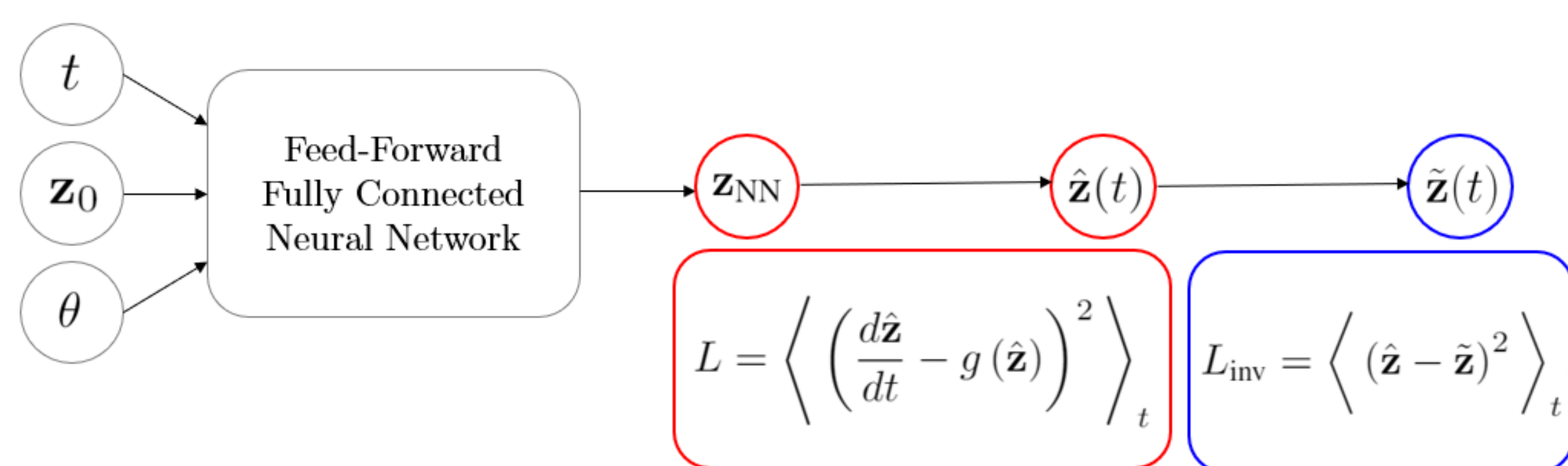
Fig. 1: Semi-supervised neural network architecture. Red and blue indicate, respectively, the unsupervised and supervised learning parts.
